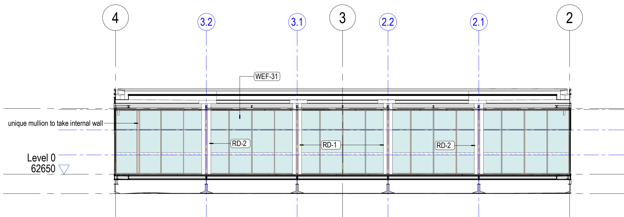
7 Courtyard West Elevation 1:100 Glazing
