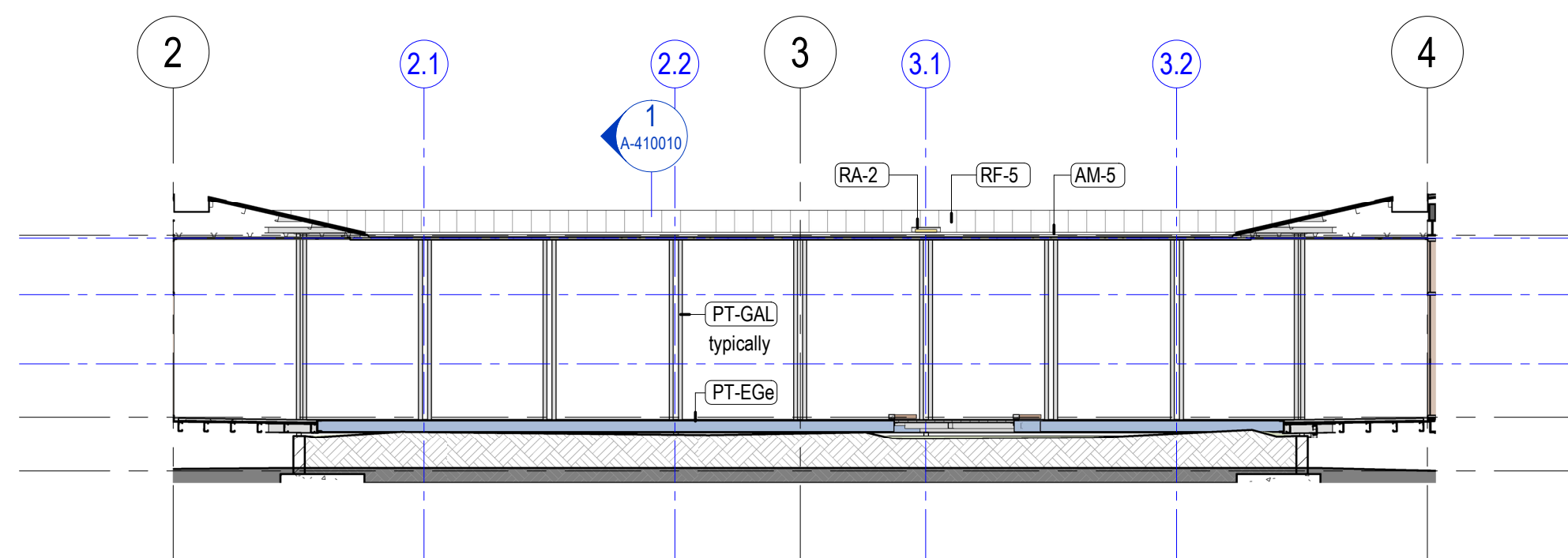
4 Courtyard East Elevation 1:100 Perimeter
