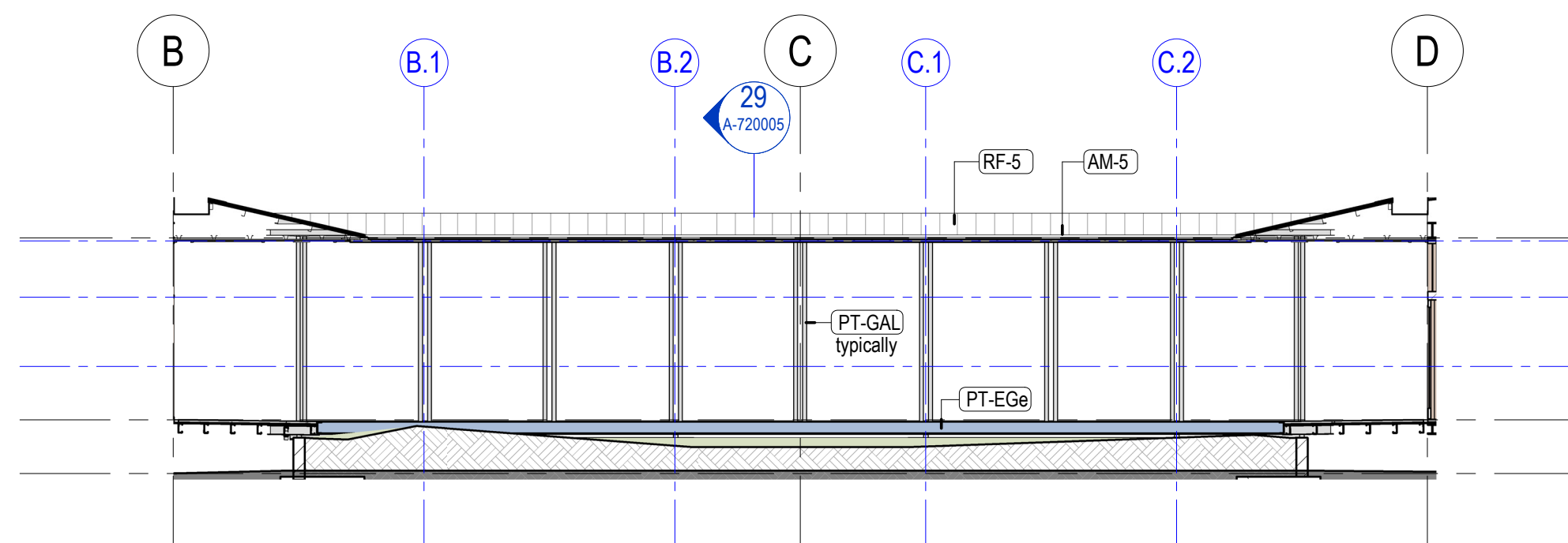
2 Courtyard North Elevation 1:100 Perimeter
