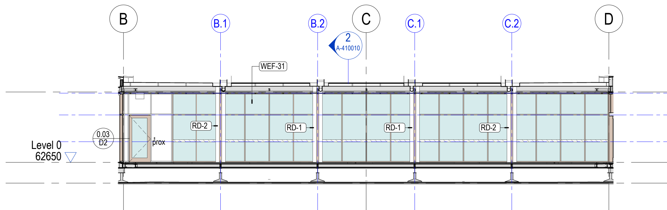
1 Courtyard North Elevation 1:100 Glazing
