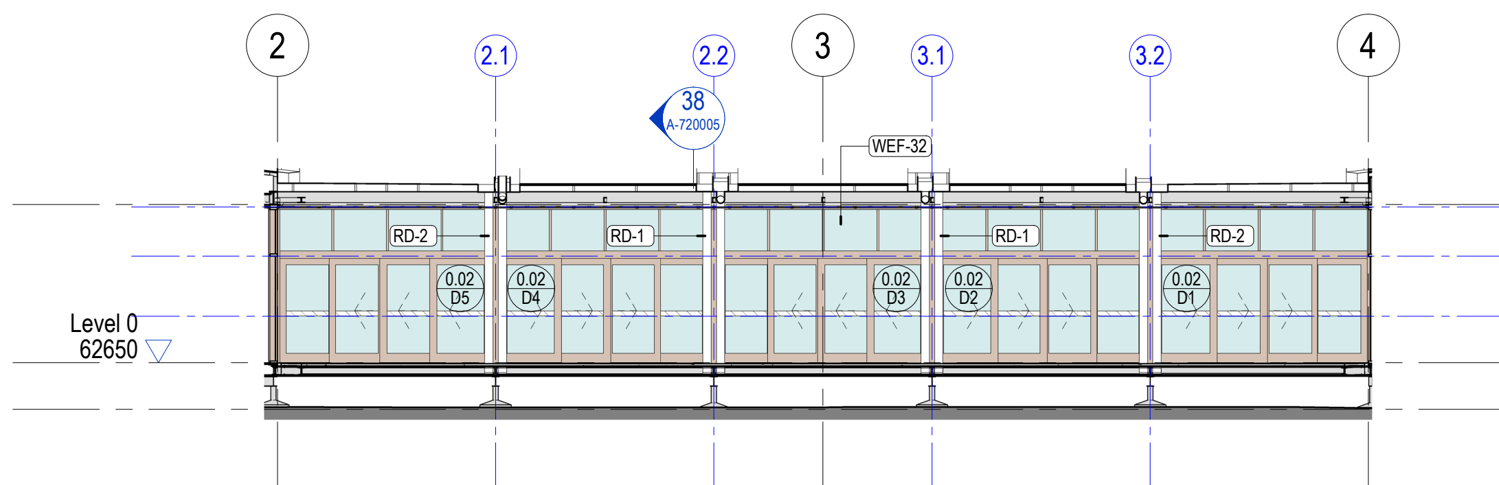
3 Courtyard East Elevation 1:100 Glazing
