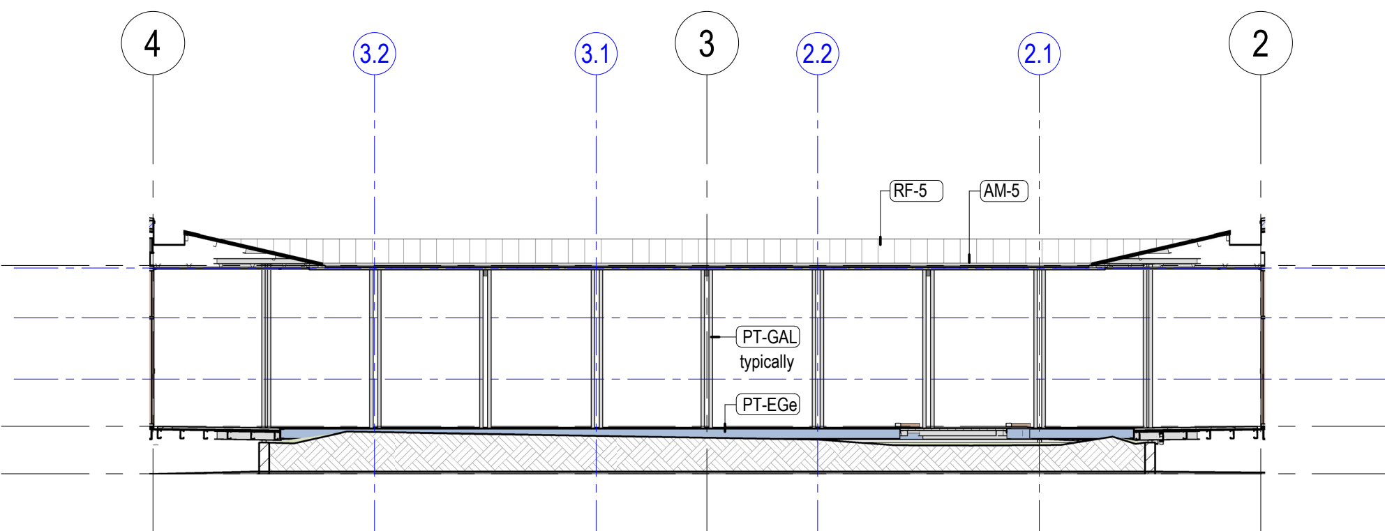
8 Courtyard West Elevation 1:100 Perimeter
