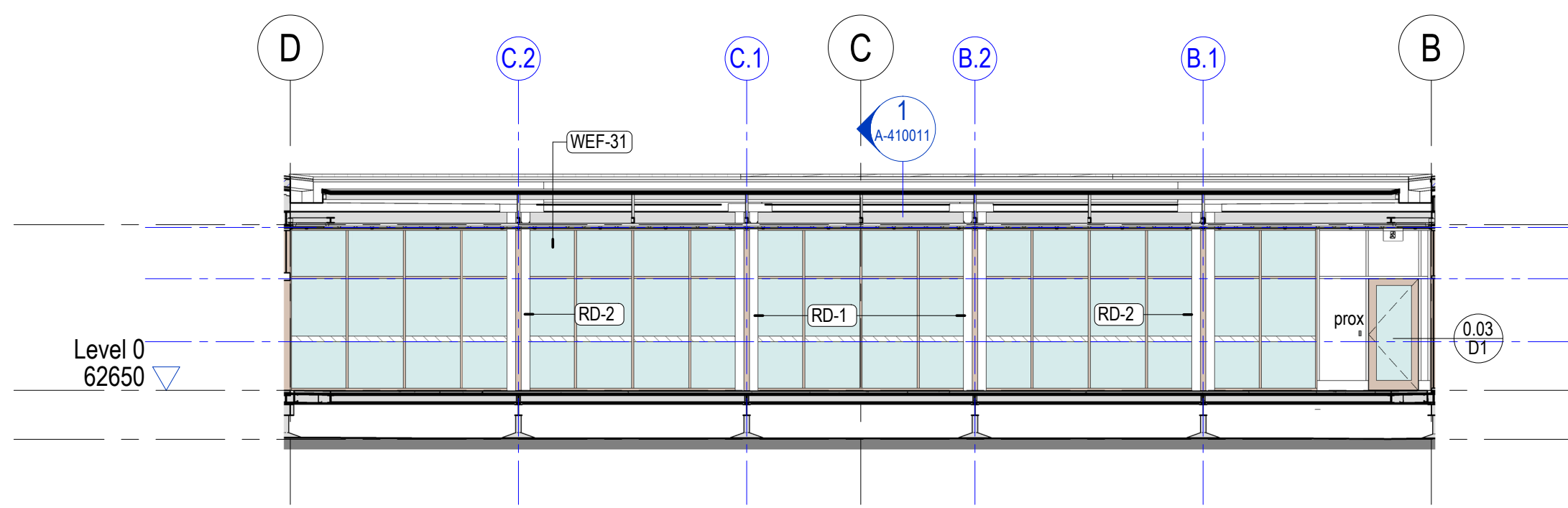
5 Courtyard South Elevation 1:100 Glazing
