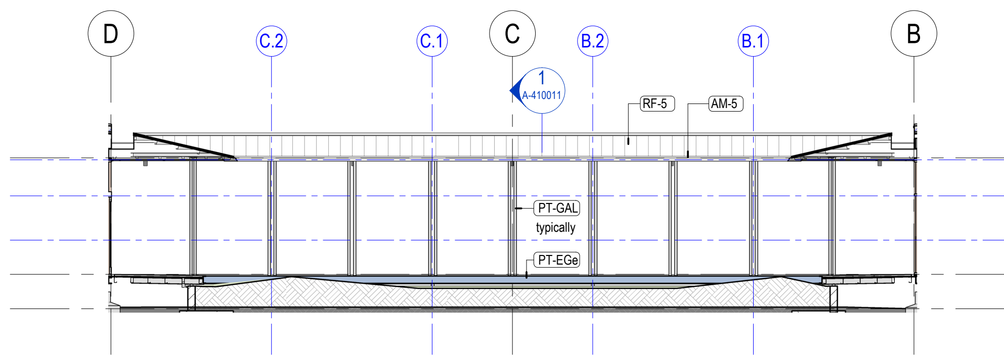
6 Courtyard South Elevation 1:100 Perimeter
